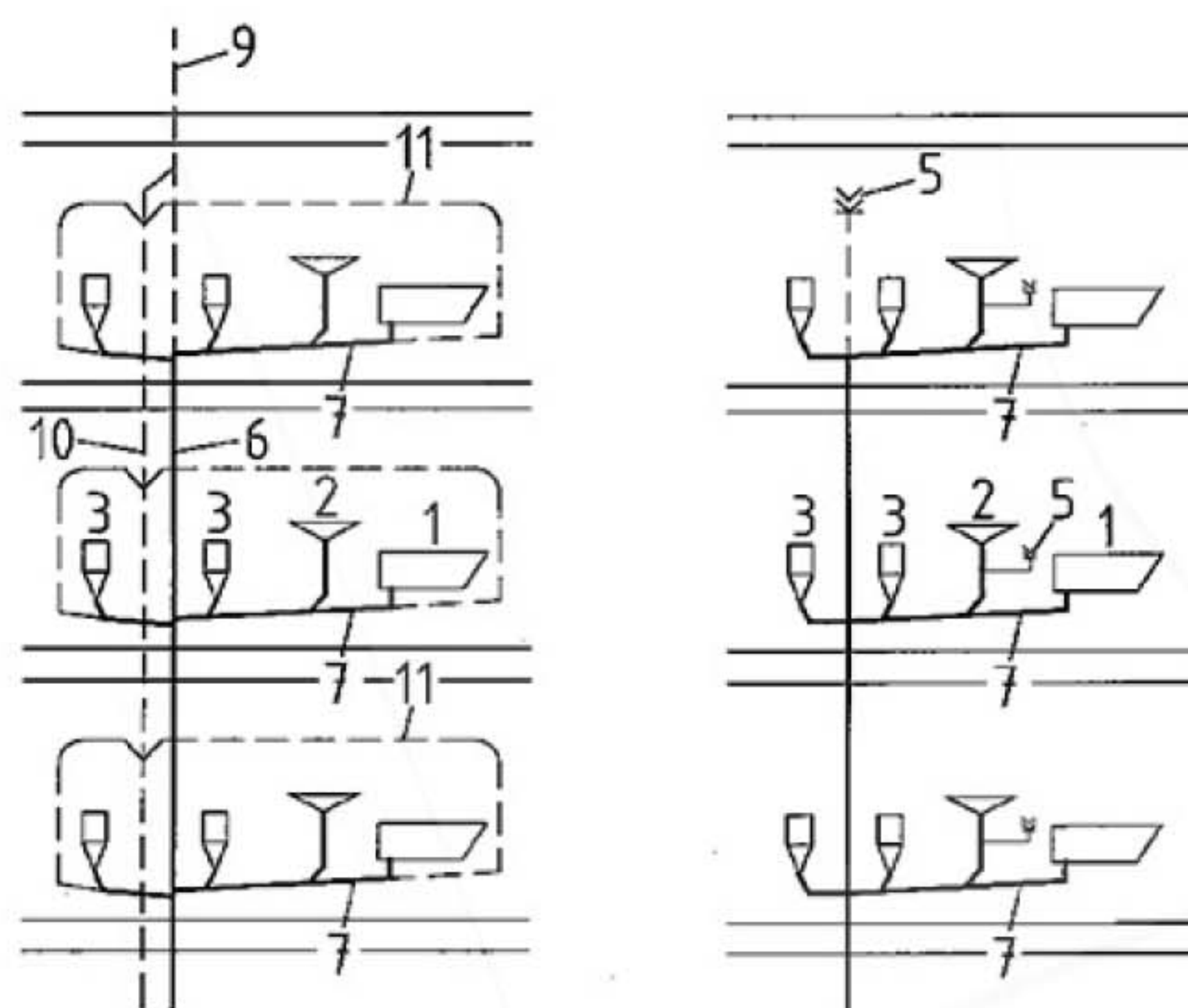
Figure 5 — Ventilated discharge branch configurations
