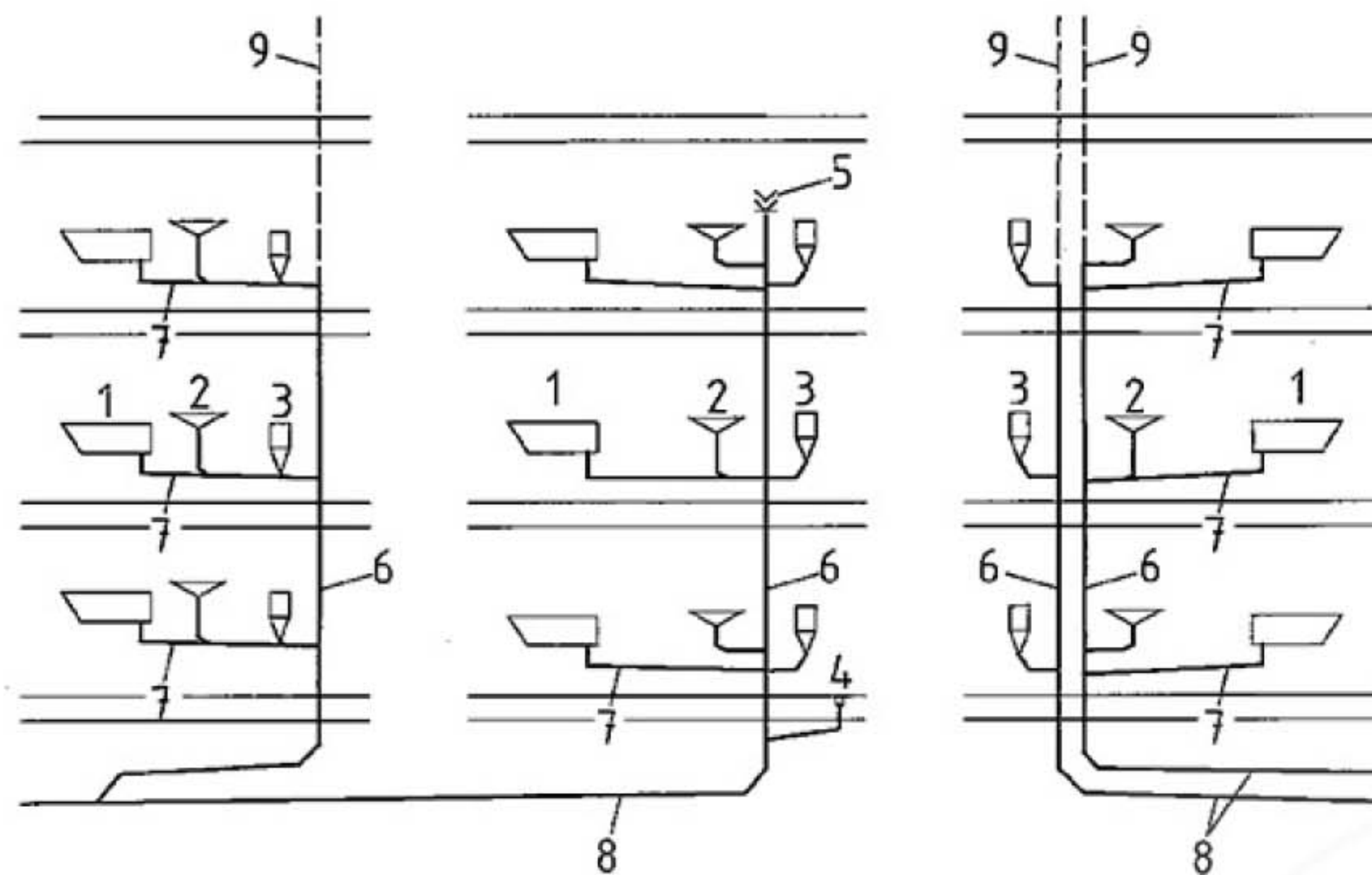
Figure 2 — Primary ventilated system configurations
